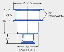
Male thread
