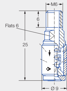
Male thread
